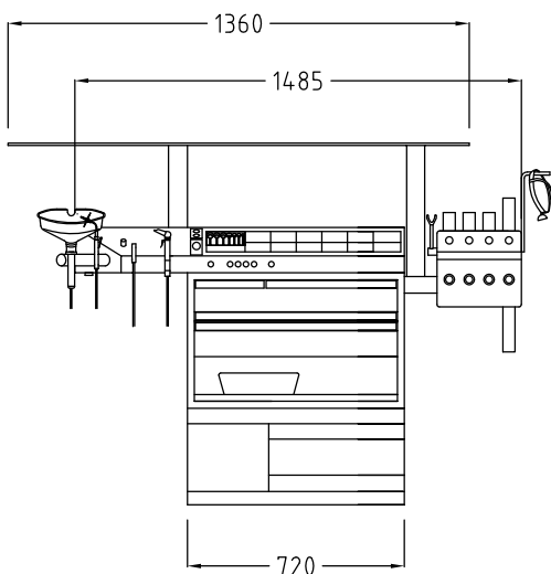
BASIC PLUS 700 with high-plateau
