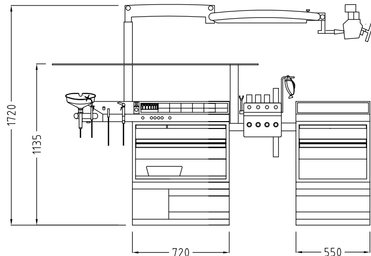
BASIC PLUS STATION with microscope and with high-plateau
