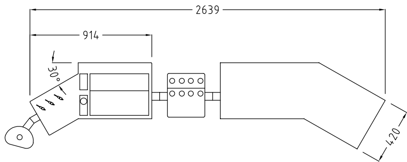
BASIC PLUS STATION with microscope and with high-plateau
