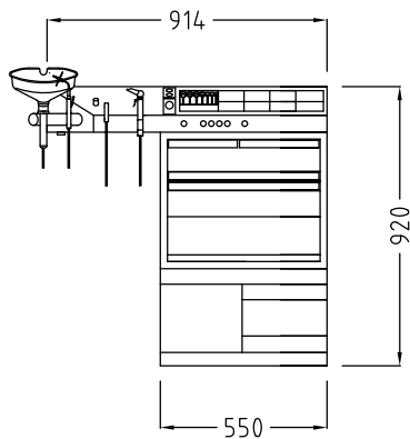
BASIC PLUS with Desk L
