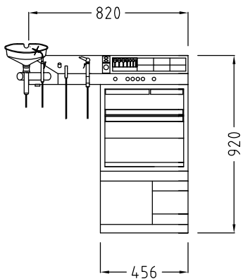
Lateral view
